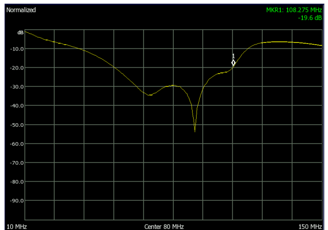
IN Returnloss (10-150MHz)
