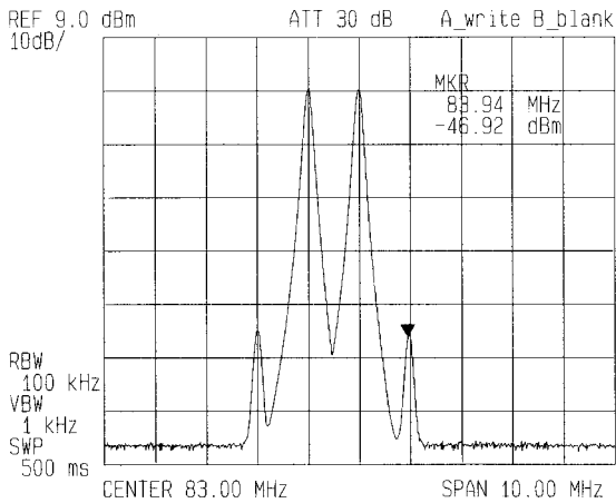
2信号特性(82MHz,83MHz) @+24
